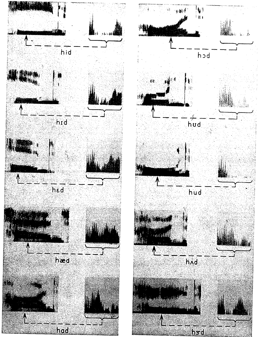
FIG. 2. Broad band spectrograms and amplitude sections of the word list by a female speaker.
