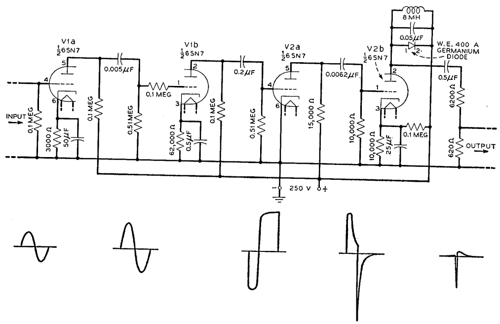
Fig. 5. Schematic of calibrating tone generator.
