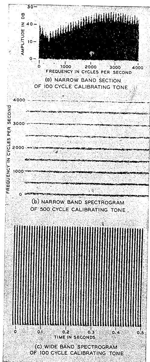
FIG. 6. Spectrograms and section of calibrating tone.
