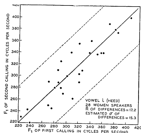
FIG. 7. Accuracy-precision chart of first formant frequencies of [i] as spoken by 28 women.
